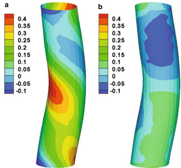
Fig. 7 Deviation of the stress ( (\sigma^k - \sigma_h^k) / \sigma_h^k ) from the target homeostatic stress in a helical fiber ( k = 4 ) without (a), and with (b), optimized distributions of thickness and anisotropy
