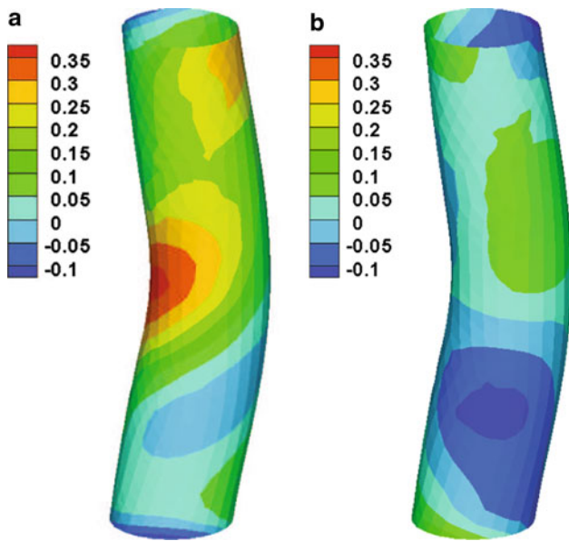
Fig. 6 Deviation of the stress ( (\sigma^k - \sigma_h^k) / \sigma_h^k ) from the target homeostatic stress in a helical fiber ( k = 3 ) without (a), and with (b), optimized distributions of thickness and anisotropy
