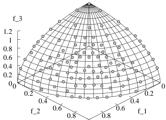
Fig. 15. \epsilon -MOEA distribution on DTLZ2.
