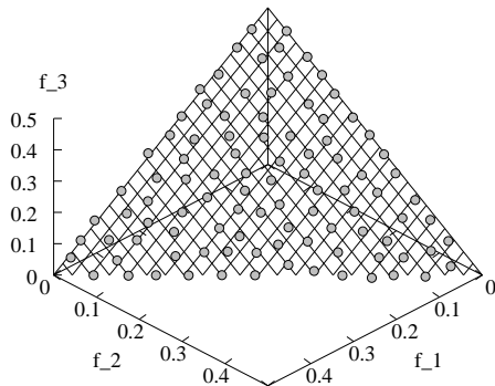
Fig. 9. C-NSGA-II distribution on DTLZ1.
