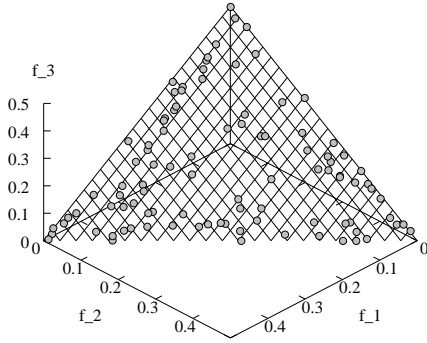
Fig. 8. NSGA-II distribution on DTLZ1.
