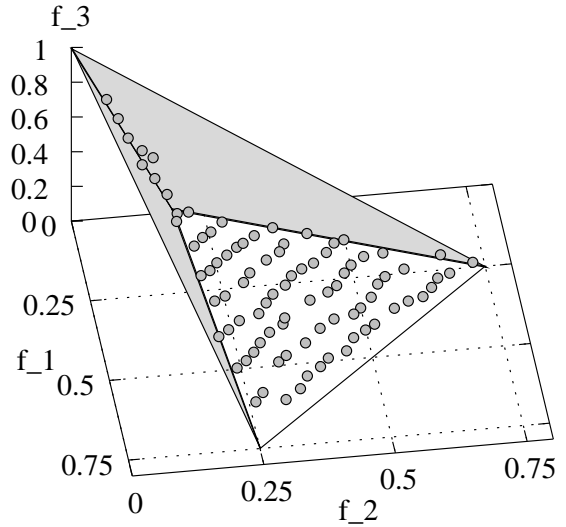
Fig. 19. \epsilon -MOEA distribution on DTLZ8.
