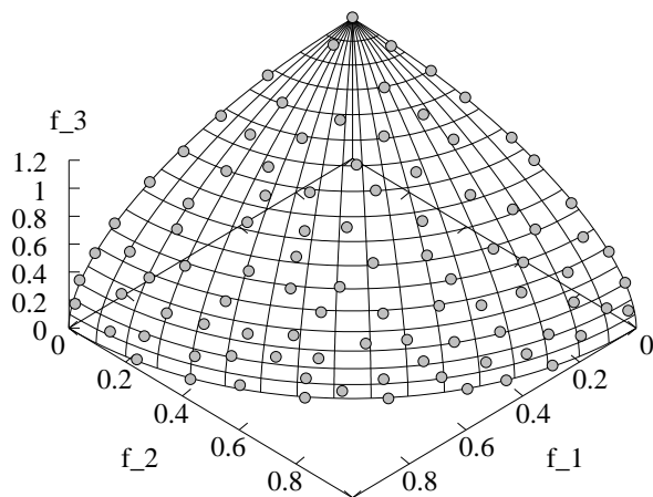
Fig. 14. C-NSGA-II distribution on DTLZ2.
