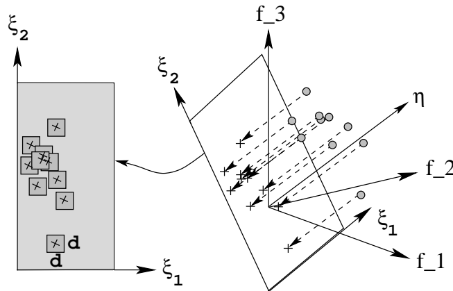
Fig. 13. The sparsity measure is illustrated.
