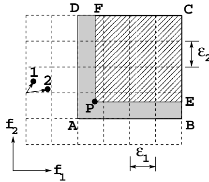
Fig. 5. The \epsilon -dominance concept is illustrated (for minimizing f_1 and f_2 ).
