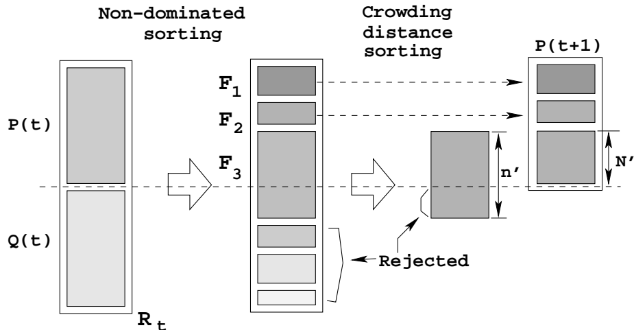
Fig. 3. NSGA-II procedure is illustrated.
