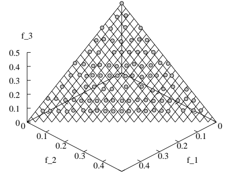
Fig. 10. \epsilon -MOEA distribution on DTLZ1.
