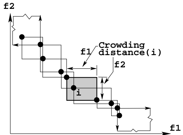
Fig. 2. The crowding approach used in NSGA-II is illustrated.
