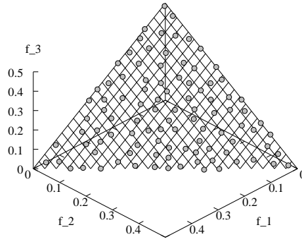
Fig. 9. C-NSGA-II distribution on DTLZ1.
