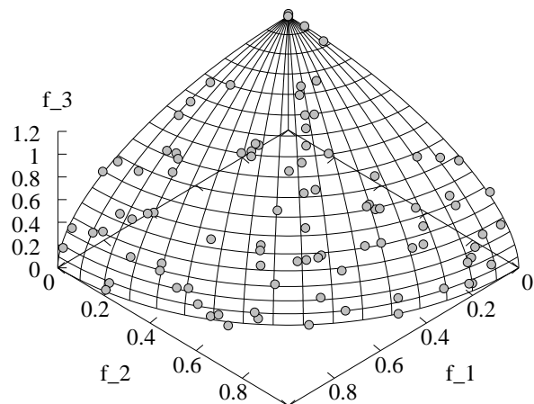
Fig. 15. \epsilon -MOEA distribution on DTLZ2.
