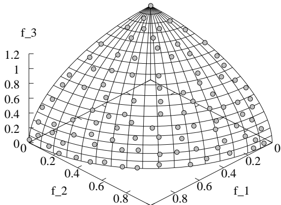
Fig. 14. C-NSGA-II distribution on DTLZ2.
