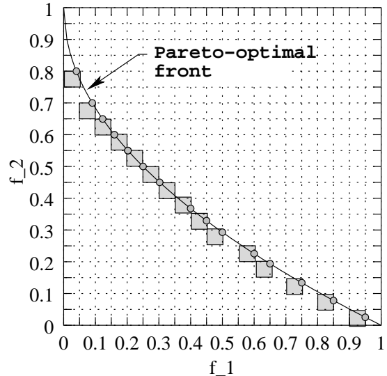
Fig. 7. \epsilon -MOEA distribution on ZDT1 with \epsilon = 0.05 .
