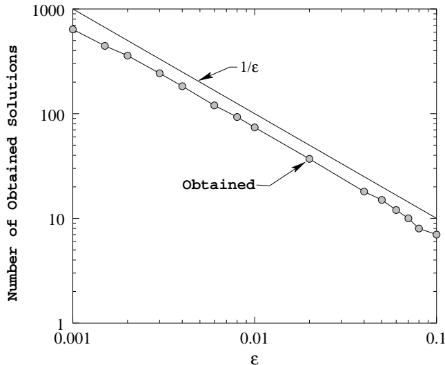
Fig. 6. The number of solutions versus \epsilon on ZDT1.
