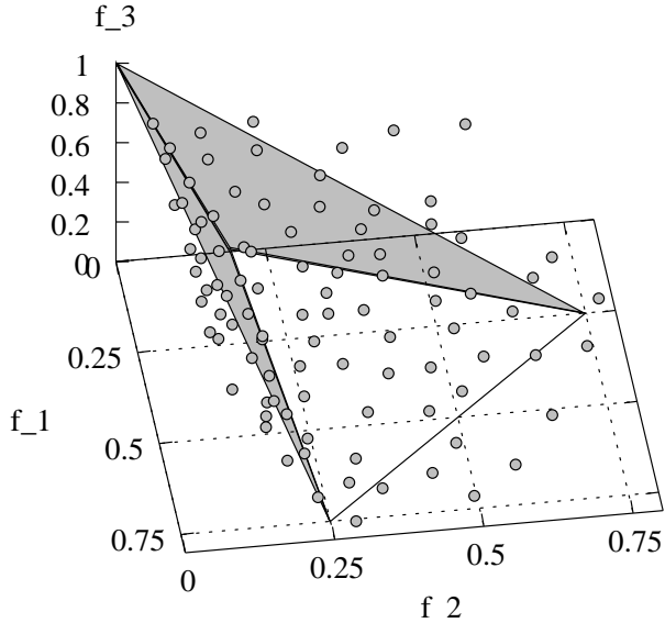
Fig. 18. SPEA2 distribution on DTLZ8.
