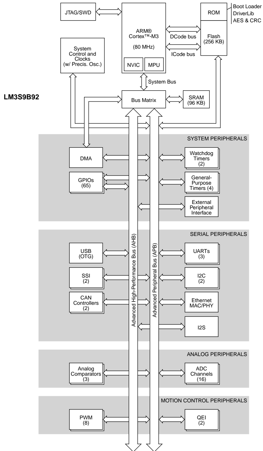
Figure 1-1. Stellaris® LM3S9B92 Microcontroller High-Level Block Diagram
