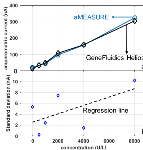
Fig. 7. a) XOx detection using aMEASURE2 compared with a benchmark GeneFluidics Helios electrochemical instrument; b) standard deviation between Helios and aMEASURE2 at each measured concentration.
