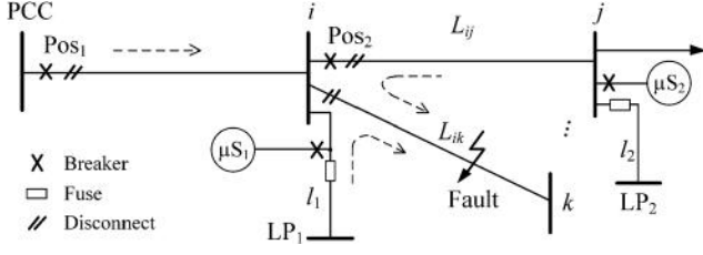
Fig. 3. Part of microgrid system.
