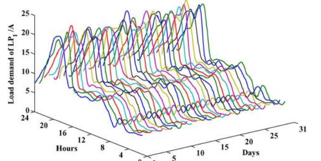
Fig. 13. Monthly load demand of LP_1 .
