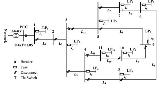
Fig. 8. Benchmark 0.4 kV microgrid network.
