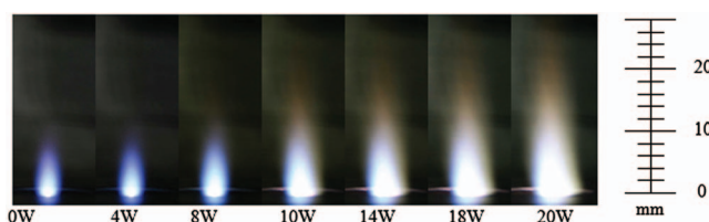
FIG. 8. (Color) Visual images of combustion flames as microwave power levels are varied from 0 to 20 W for flow rates of 49/98 SCCM \text{CH}_4/\text{O}_2 . The gap length is L_g=1 mm below the x=0 .
