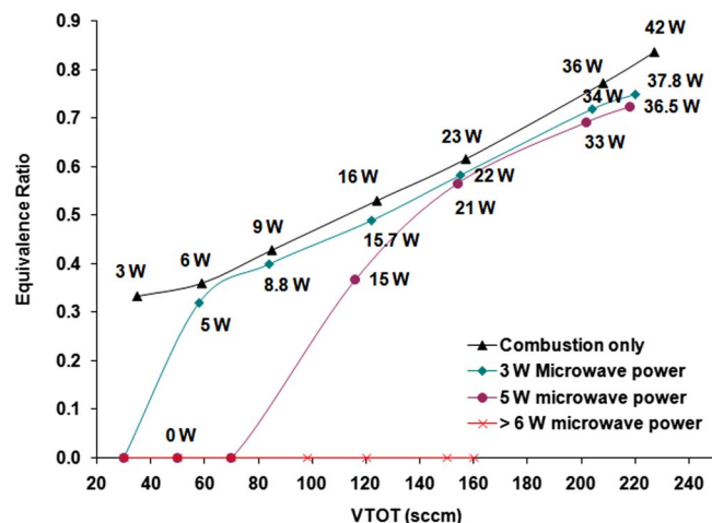
FIG. 12. (Color online) Flame extinction curves for combustion flames with 0, 3, 5, and 6 W additional of microwave power. The corresponding combustion power is displayed for each data point.
