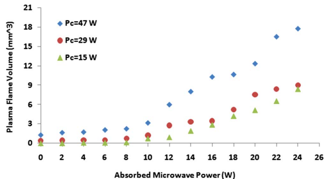
FIG. 11. (Color online) Plasma flame volume with increasing microwave energy at various total flow rates with its corresponding combustion power. P_c is the combustion power at each flow rate.
