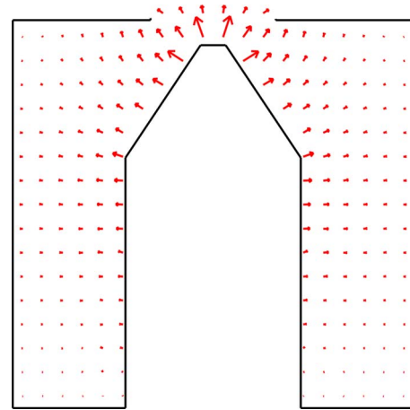
FIG. 5. (Color online) Numerically calculated relative electric field distributions inside the coaxial applicator with no flame/discharge present. The lengths of the arrows indicate the relative magnitude of the electric field strength. Frequency=2.45 GHz, cavity ID=3.2 cm, L_s=3.1 cm, inner conductor OD=1.2 cm, and L_g=2 mm.
