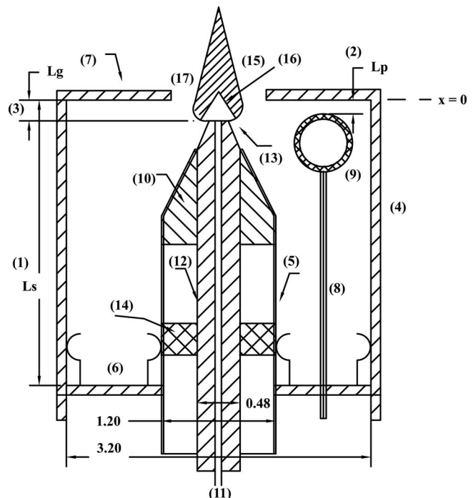
FIG. 4. The cross-section of the microwave re-entrant coaxial cavity applicator.
