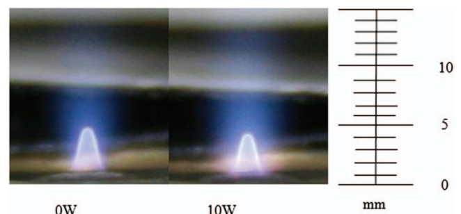
FIG. 9. (Color) Visual images of the inner cone premixed flame reaction zone with increasing microwave power at flow rates of 70/140 SCCM \text{CH}_4/\text{O}_2 .
