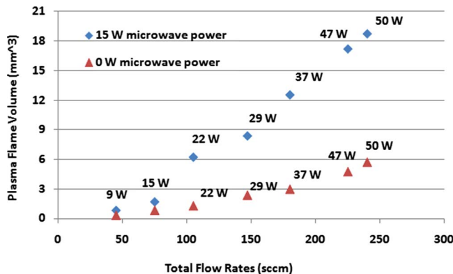
FIG. 10. (Color online) Plasma flame volume vs total flow rates at 0 and 15 W microwave power with its corresponding combustion flame power.
