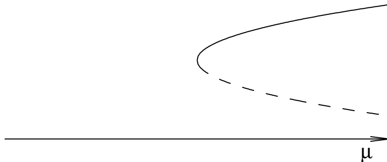
(a) Saddle–node bifurcation
