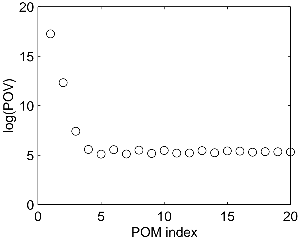
Figure 3: The logarithms of the POVs. Random noise has been added to the displacement signals.
