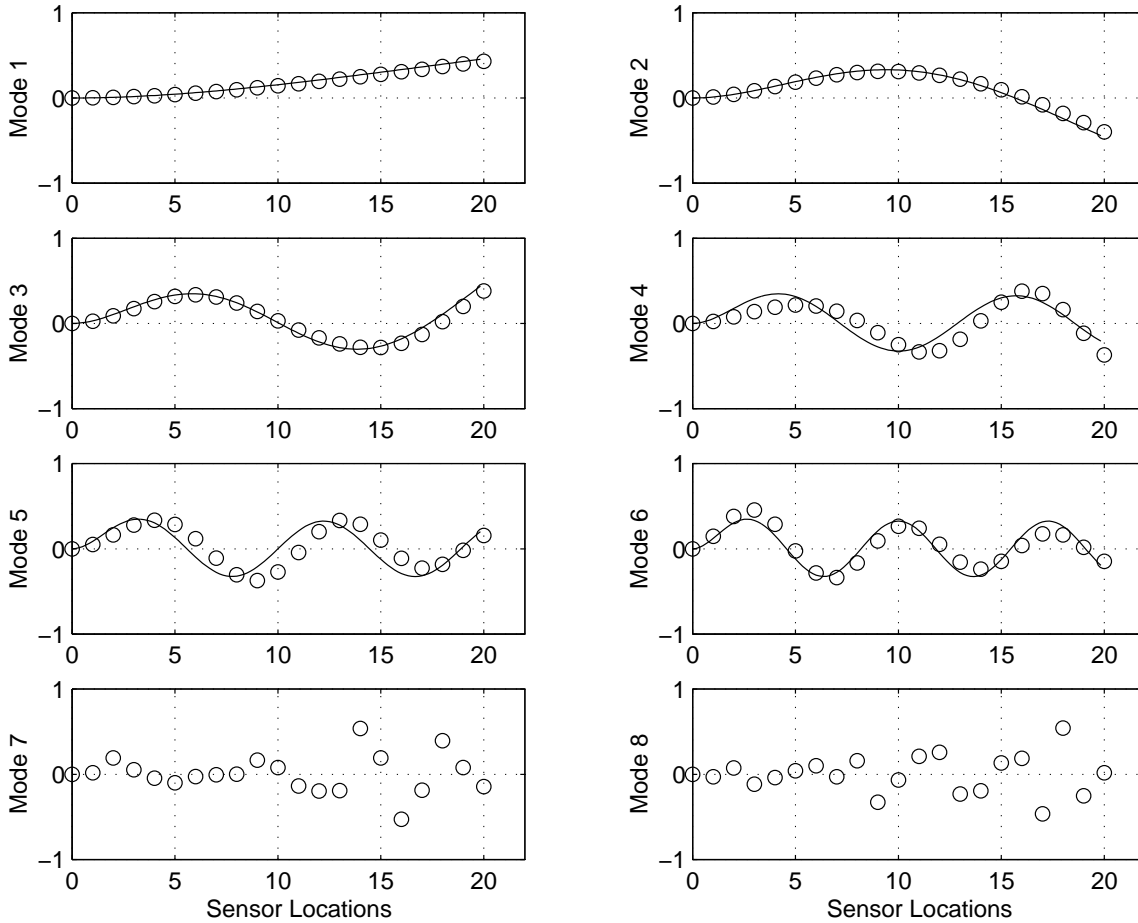
Figure 2: The first 8 POMs ordered by descending POVs. The circles indicate the POMs, and the solid lines show the theoretical normal modes.
