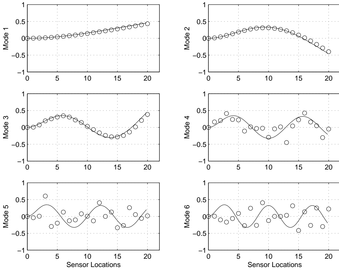
Figure 4: The first 6 POMs ordered by descending POVs for the case with added random noise. The circles indicate the POMs, and the solid lines show the theoretical normal modes.
