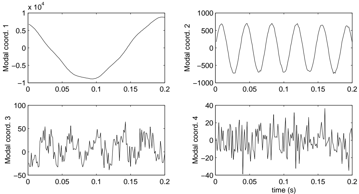
Figure 7: The proper modal coordinate histories for the first four proper orthogonal modes. In this case there is noise added to the displacement data.
