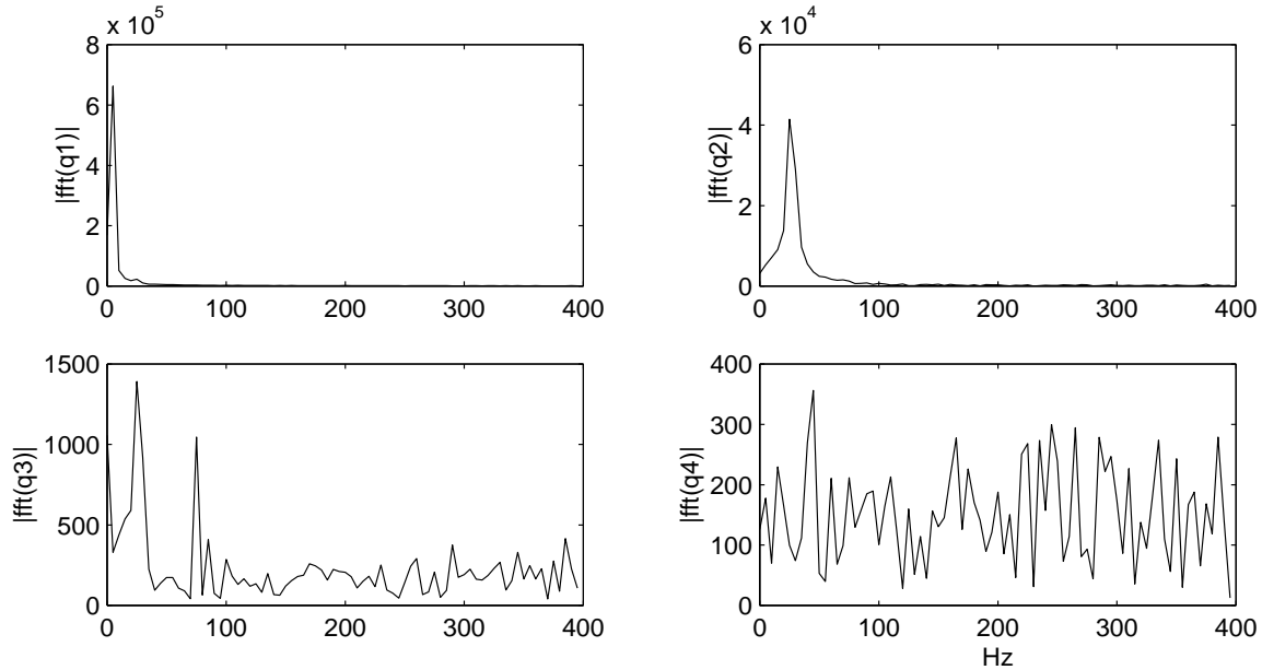
Figure 8: The Fourier transforms of the noise-contaminated proper modal coordinate histories q_i(t) for the first four proper orthogonal modes.
