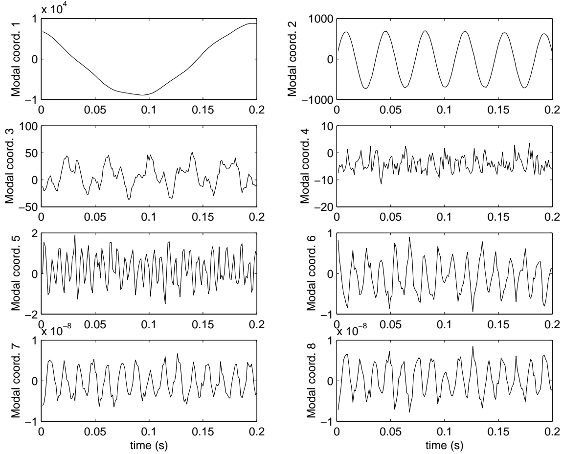
Figure 5: The proper modal coordinate histories for the first eight proper orthogonal modes.
