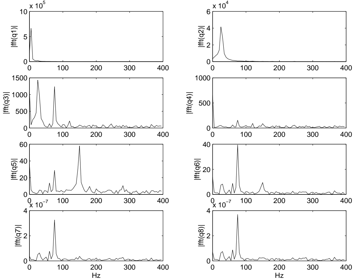
Figure 6: The Fourier transforms of the proper modal coordinate histories q_i(t) for the first eight proper orthogonal modes.
