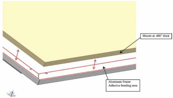
Figure 1. Faces of adhesive bonding (exploded view)
